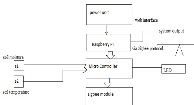
Figure 4: An operating system of Irrigation process by using Raspberry Pi
