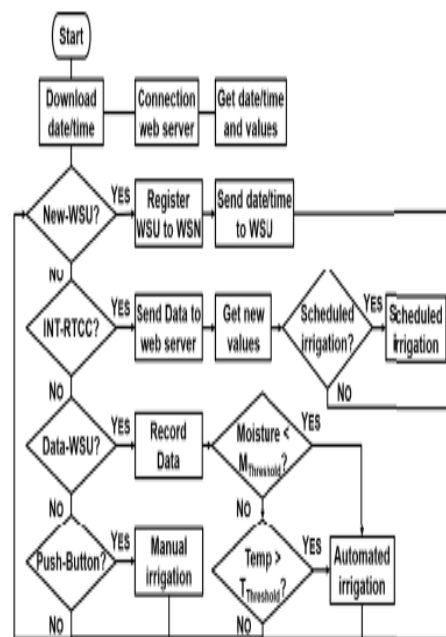
Fig 3. Algorithm of the master microcontroller in the WIU
