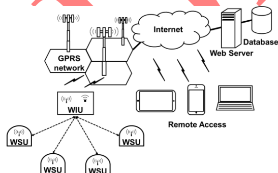
Fig. 1. Configuration of the automated irrigation system
