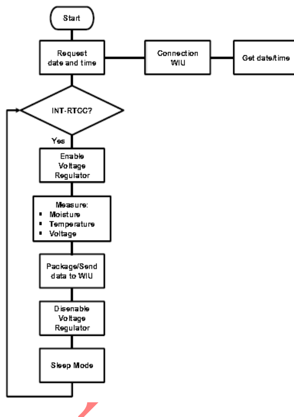
Fig. 2. Algorithm of wireless sensor unit (WSU)
