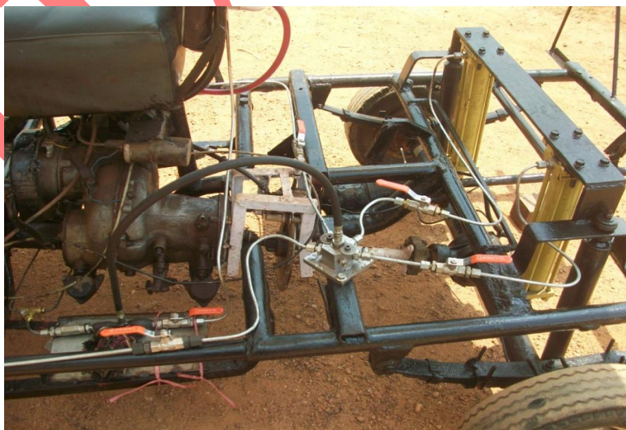
Figure 12. Photo of the Automatic Hydraulic Jack System.
