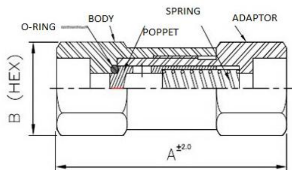
Figure 10. Non-Return Valve.
