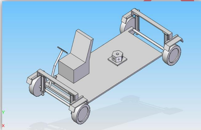
Figure 11. 3-D View of the Automatic Hydraulic Jack System.
