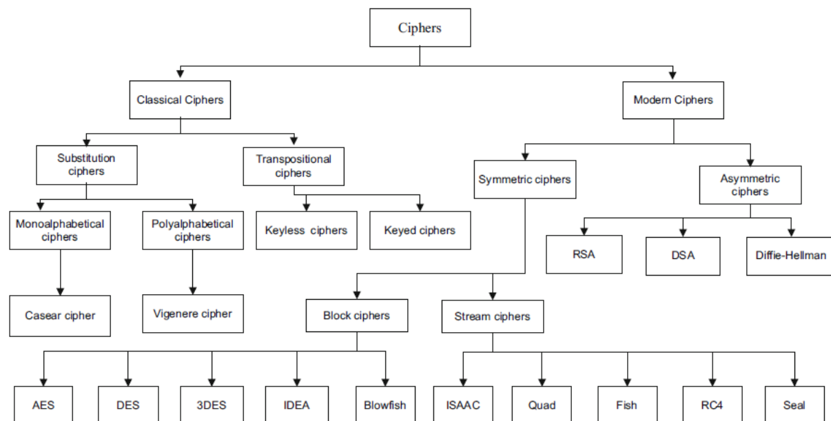
Figure: Classifications of cryptography algorithm.
