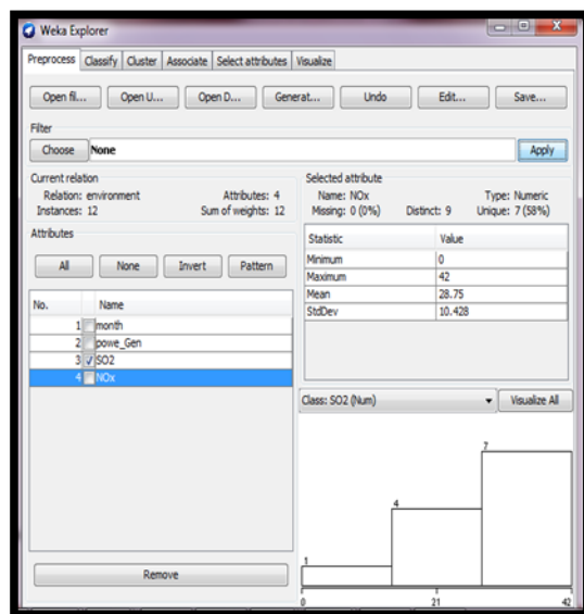
Fig:3 pre-processing the environmental data
