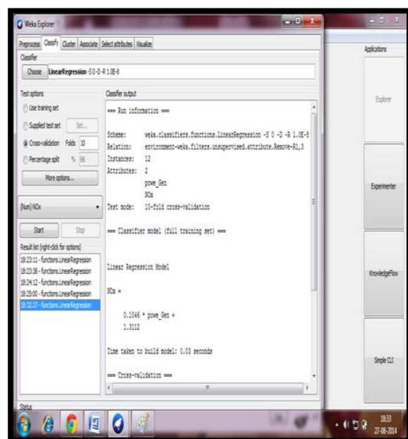
Fig:5 Linear regression for Pollutant NOx
