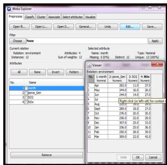
Fig: 2 loading a dataset into WEKA
