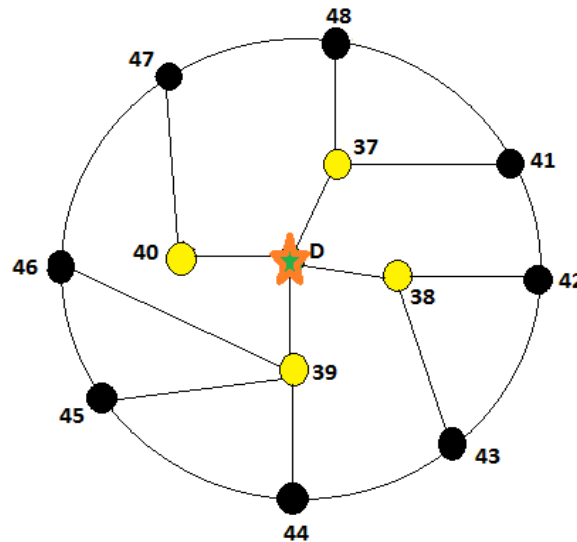
Figure 5: Final Path selection in the proposed model
